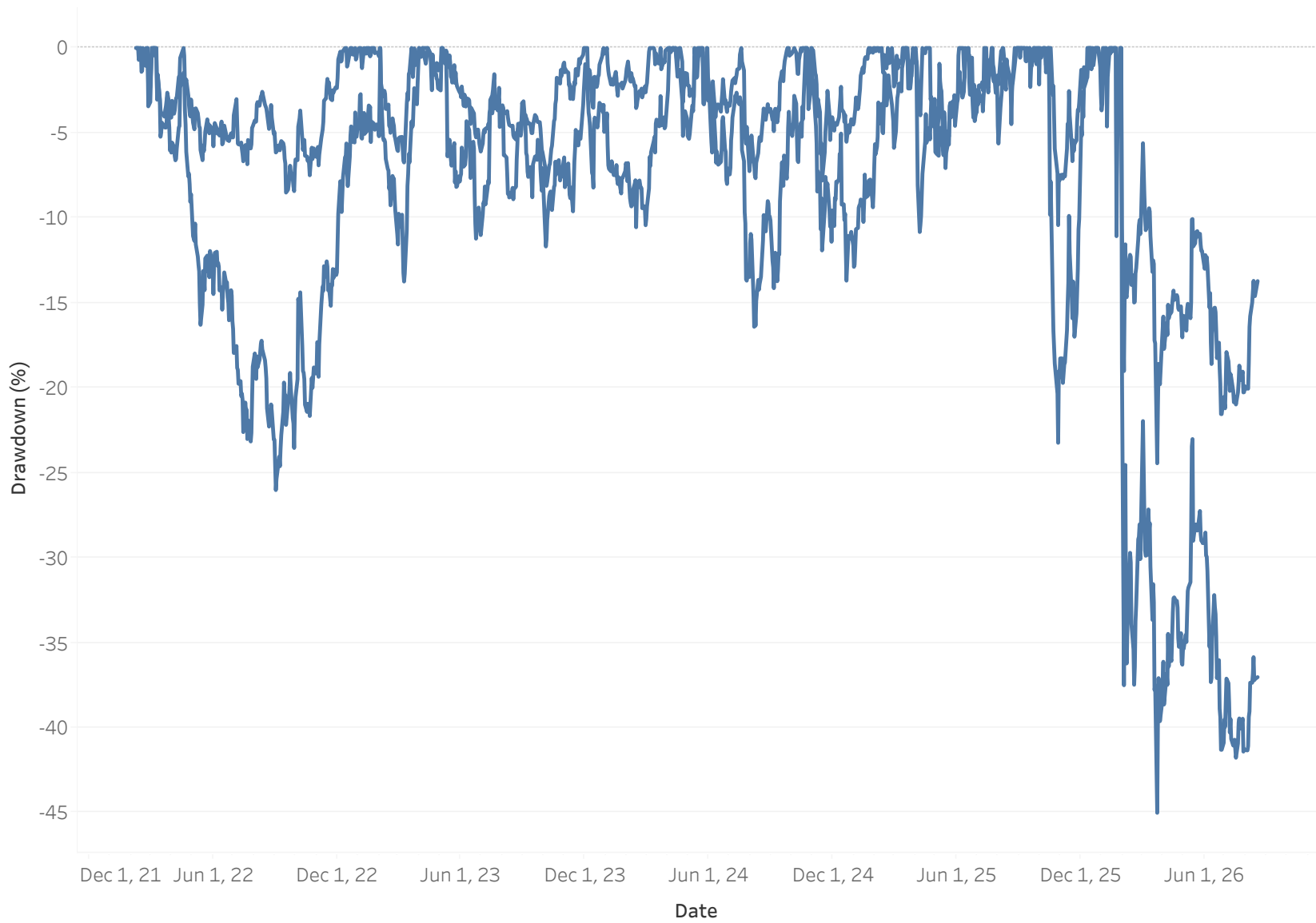
The trends of Drawdown Gold and Drawdown Silver for Date. Details are shown for Drawdown Gold and Drawdown Silver.
