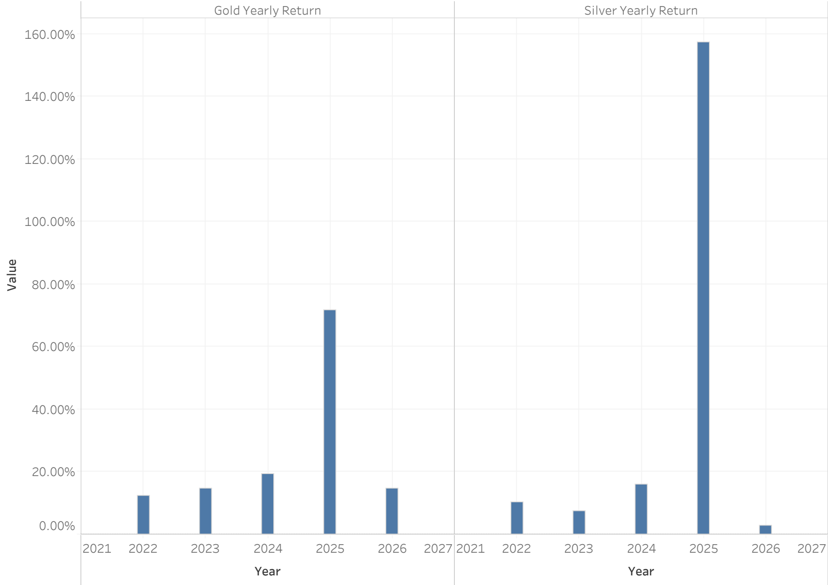
The plots of Gold Yearly Return and Silver Yearly Return for Year. Details are shown for Gold Yearly Return and Silver Yearly Return.
